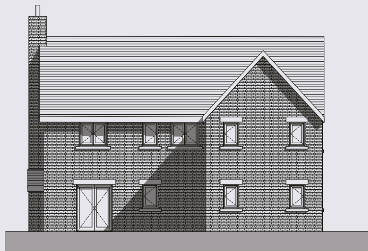
Rear - North Elevation
