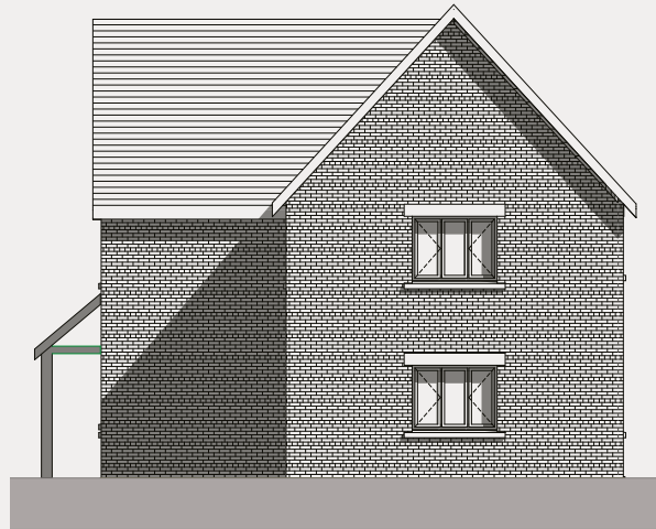
North Elevation
