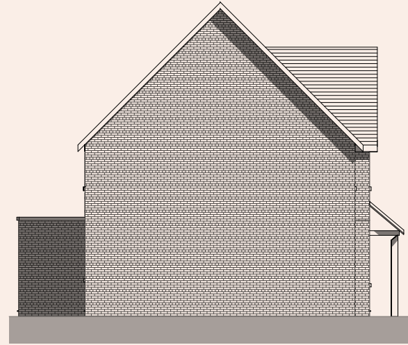
Side - North Elevation
